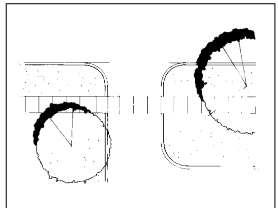
Figure 5.20 – Sidewalk material continuing across driveway curb cuts when the sidewalk is at grade with the driveway.
