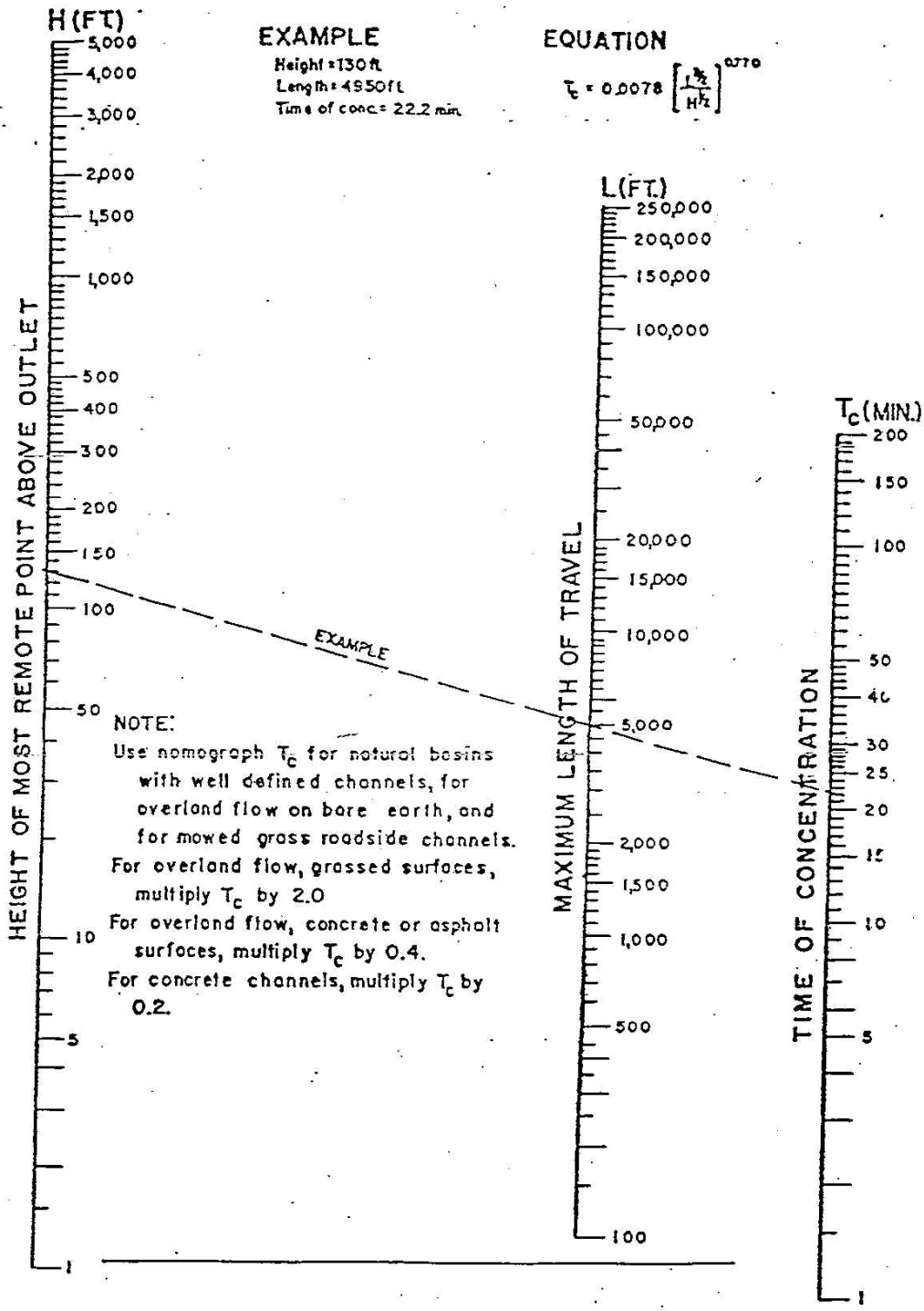
Figure 4-13: Time of Concentration Nomograph.
