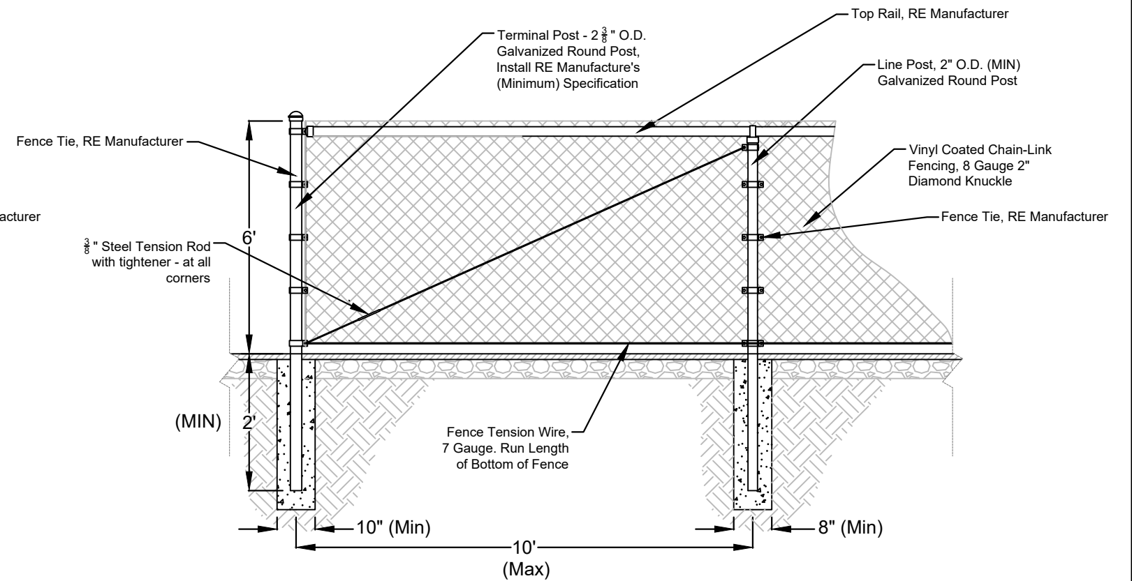
12-FOOT FENCE ELEVATION DETAIL
