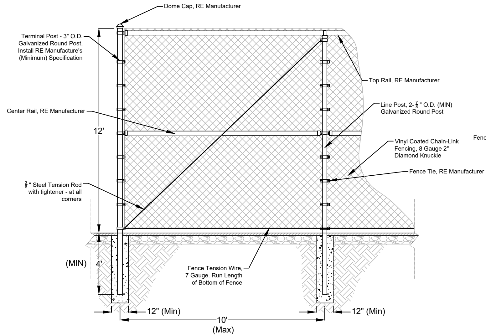
12-FOOT FENCE ELEVATION DETAIL
