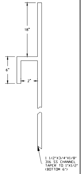
LEVEL ⑦ INSTRUMENTATION SUPPORT N.T.S.
