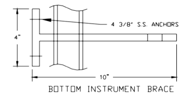
LEVEL ⑦ INSTRUMENTATION SUPPORT N.T.S.
