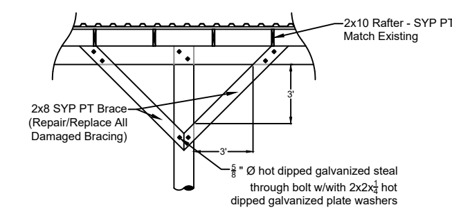
1 01 TYPICAL "Y" BRACING CROSS SECTION
