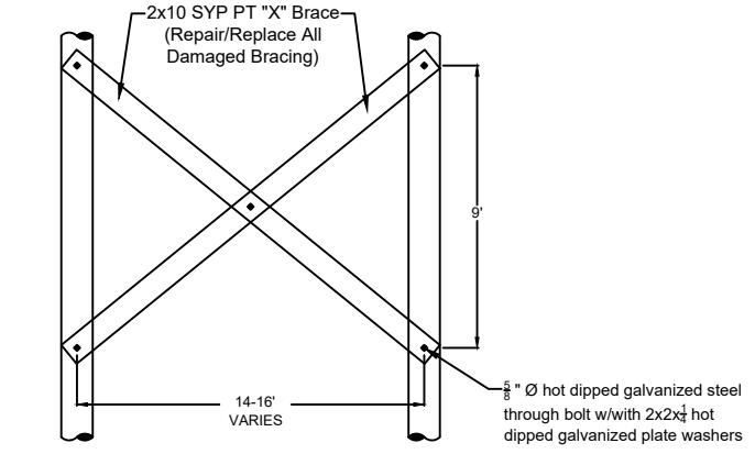
2 01 TYPICAL "X" BRACING CROSS SECTION
