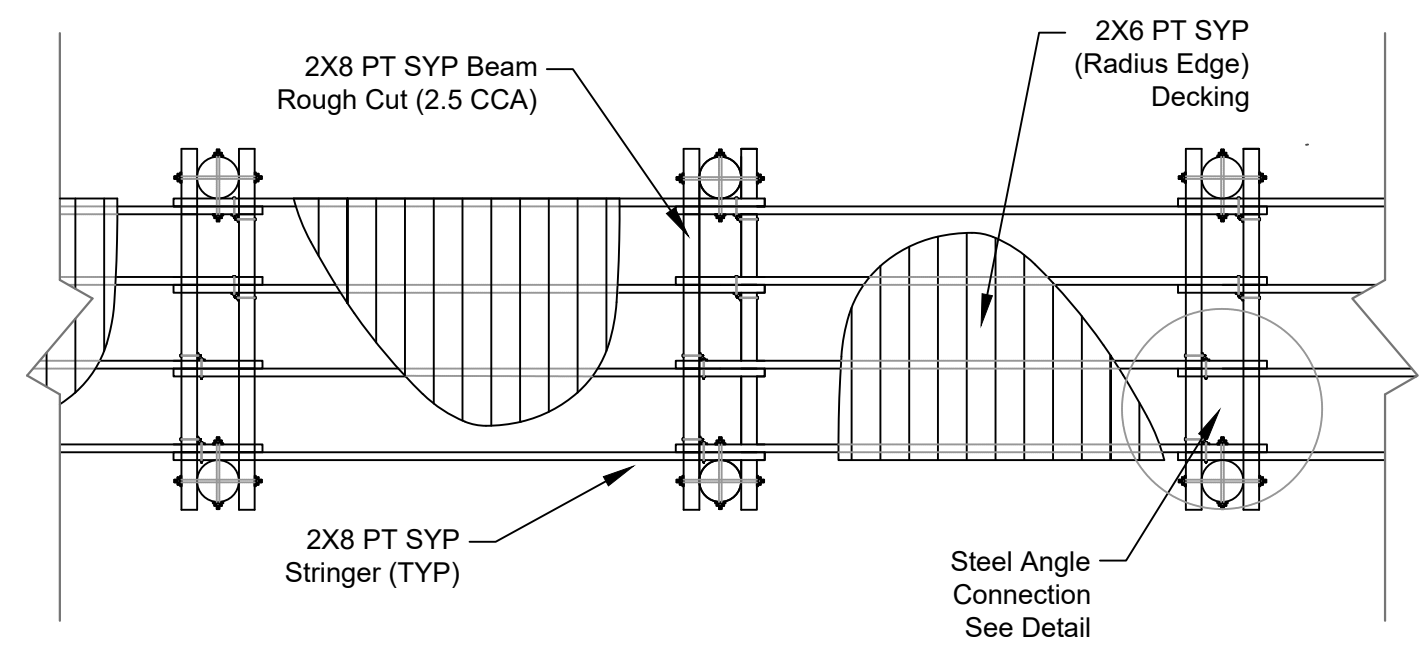
2 06 TYPICAL PIER PLAN VIEW
