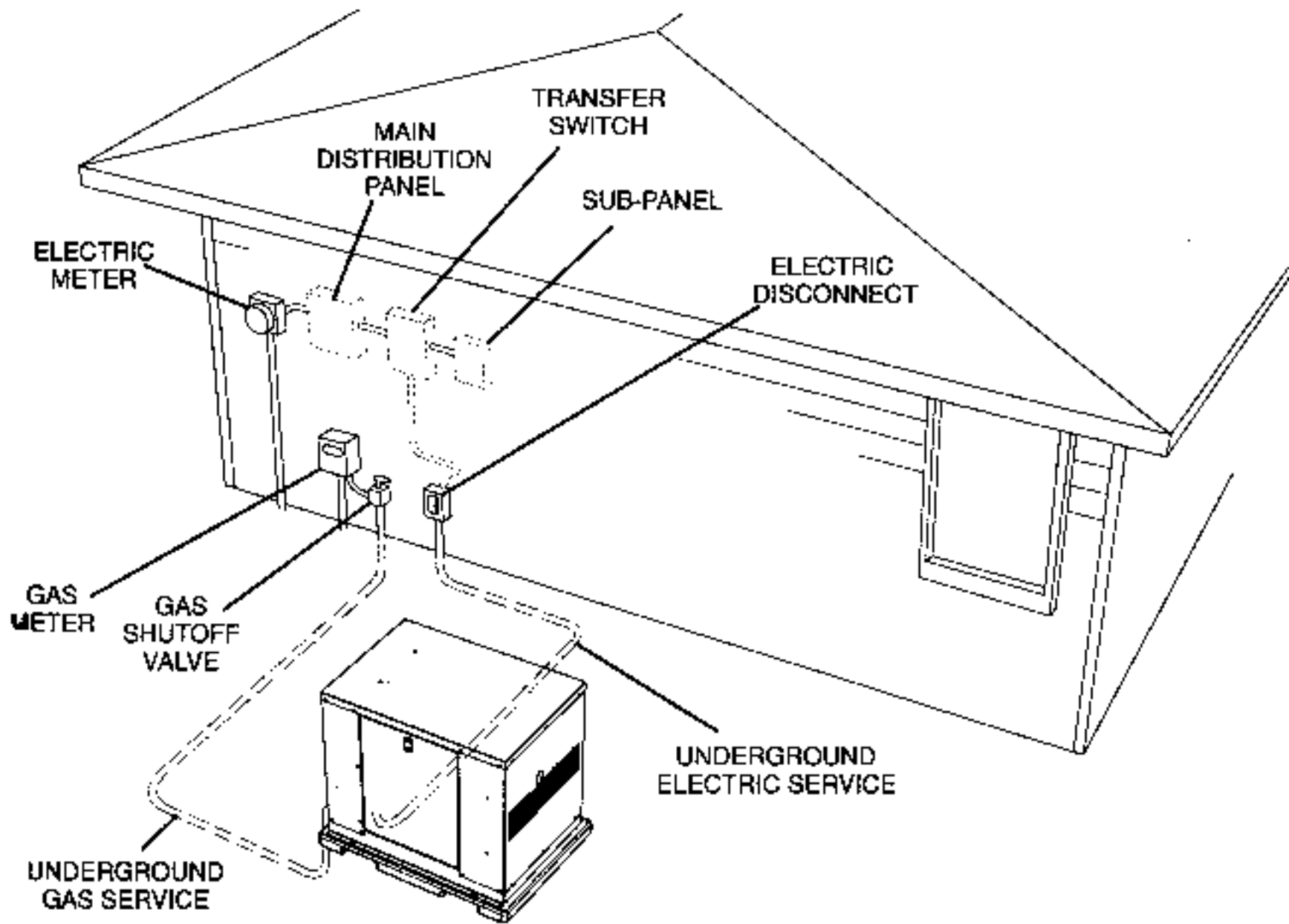
TYPICAL GENSET SITE
