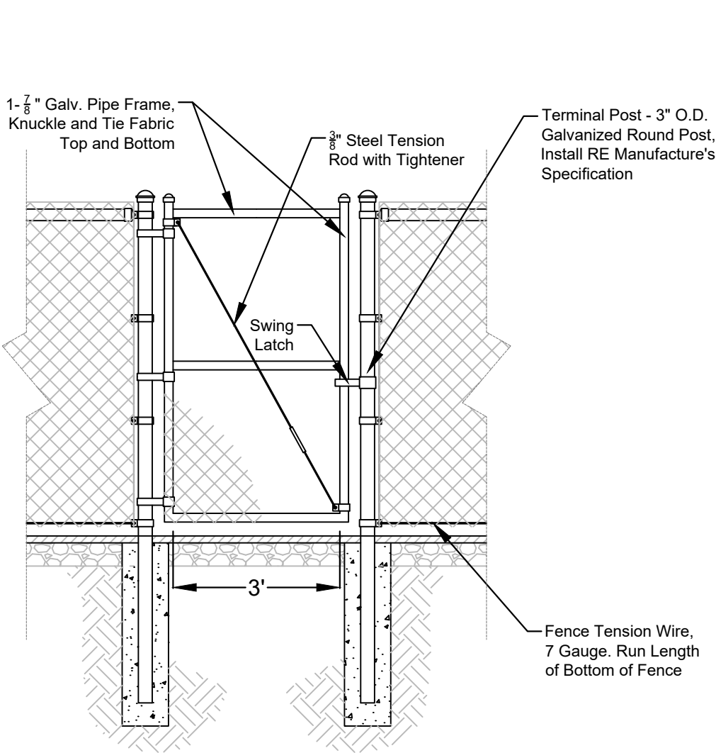
PERSONNEL GATE DETAIL
