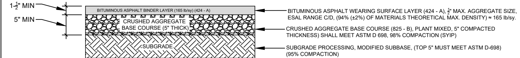
TYPICAL ASPHALT COURT SECTION NOT TO SCALE
