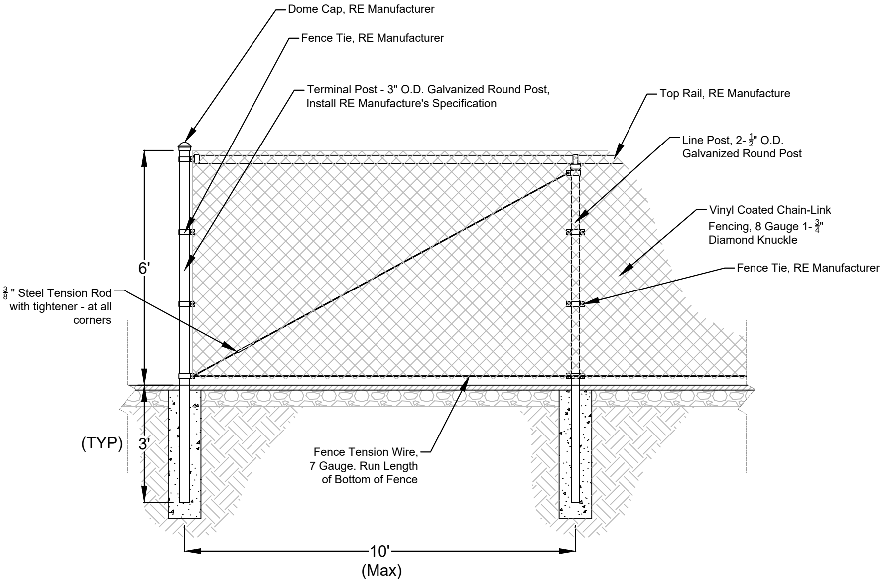
FENCE ELEVATION DETAIL
