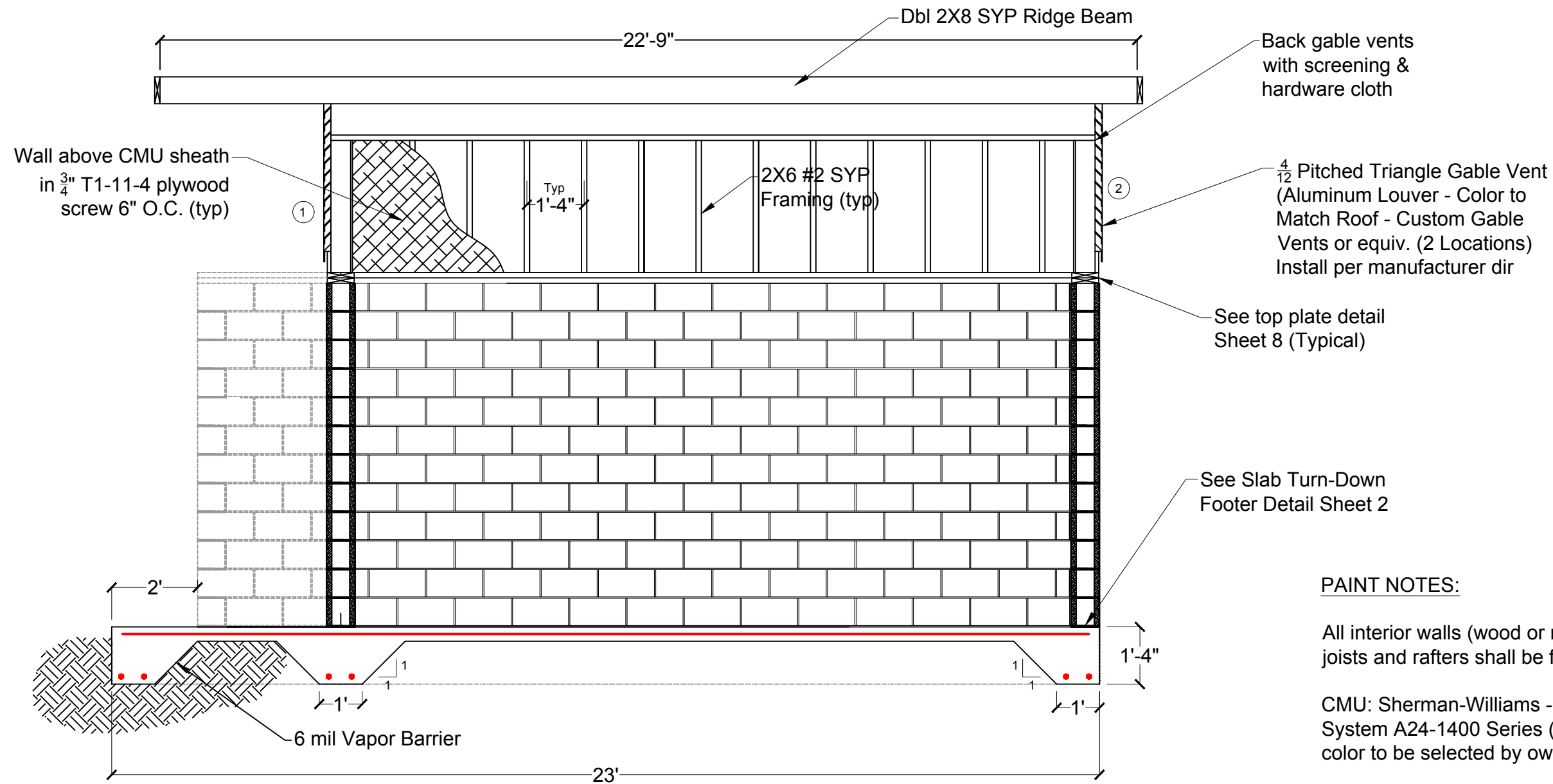
SECTION B-B ELEVATION VIEW
